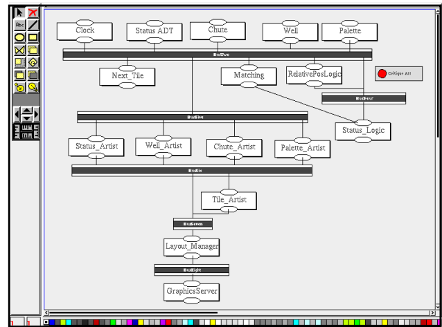
Figure 2. Conceptual Architecture Perspective
