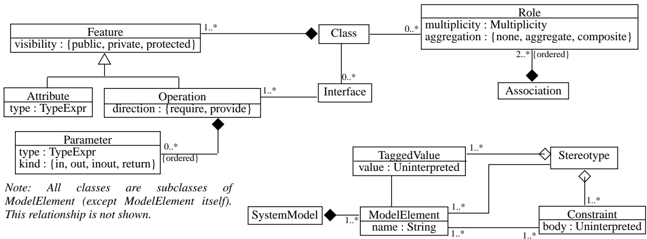
Figure 3. Simplified UML Meta-Model (Adapted from [18])
