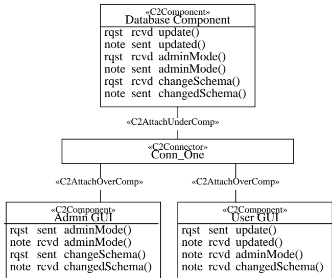
Figure 5. An example C2-style architecture for a database
