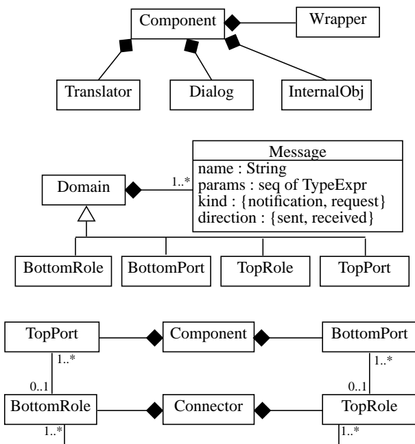
Figure 4. A meta-model for C2-style architectures
