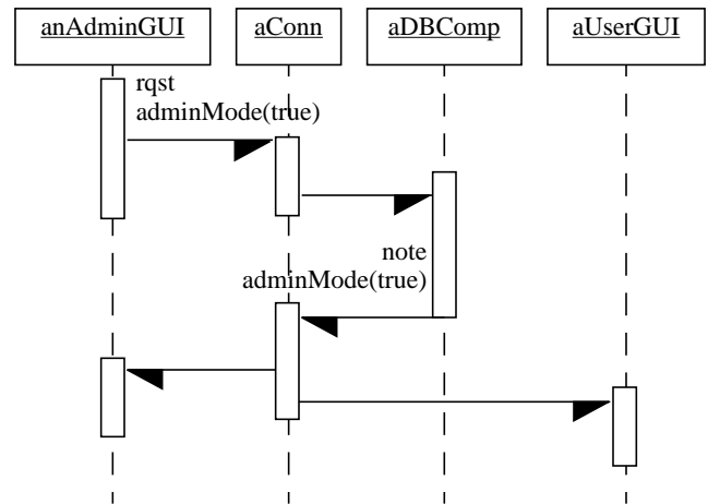
Figure 7. Sequence diagram for Disable User Access
